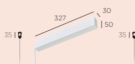
base B32
